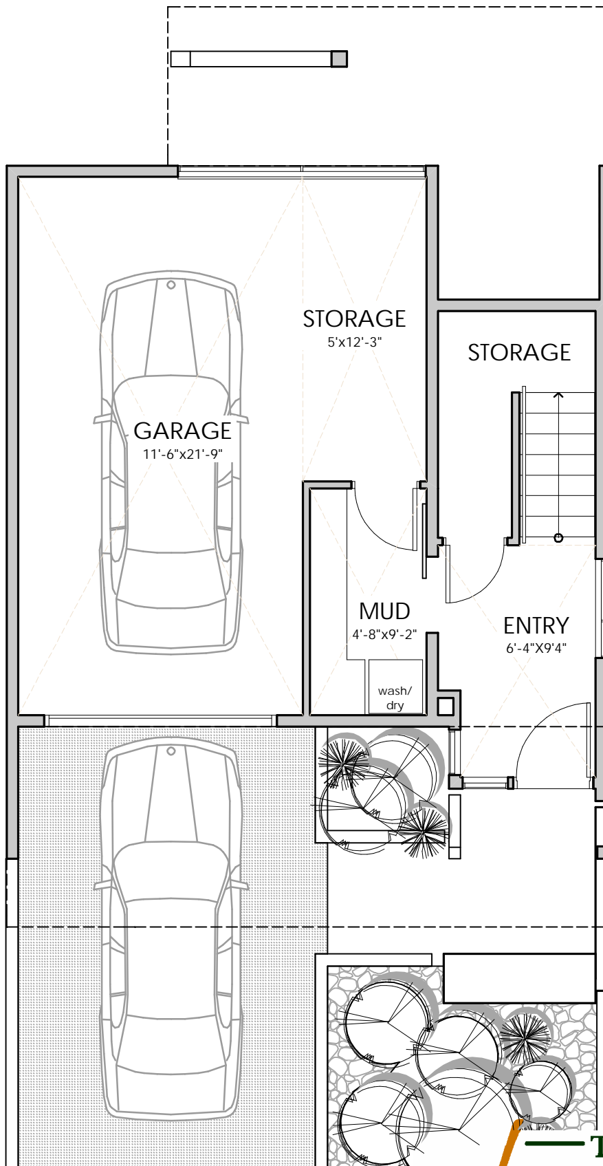
GROUND FLOOR PLAN 3/16"=1' @ 8½x11" paper size
